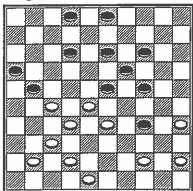
Diagram 5 - Forcing
